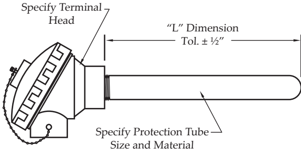
STYLE TPT - Metal Protection Tube
