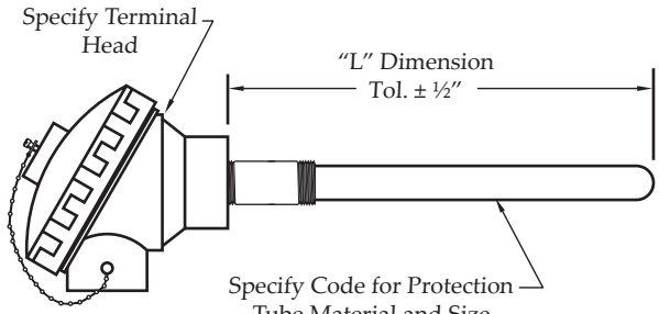
STYLE TPTC - Ceramic Protection Tube with Pipe Nipple
