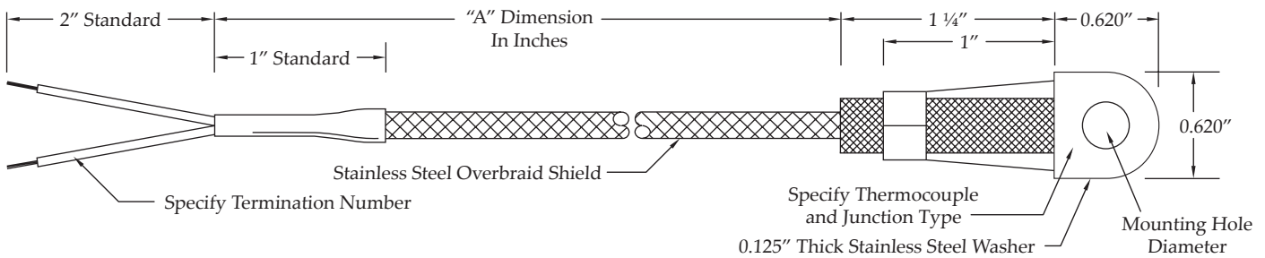
TSM2 - Gasket with Bracket Leadwire Conductor is Stranded with Fiberglass Insulation and Stainless Steel Overbraid Shield
