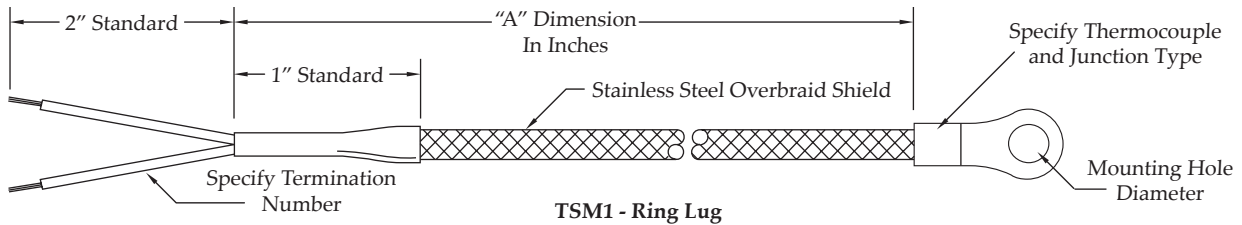
TSM1 - Ring Lug Leadwire Conductor is Stranded with Fiberglass Insulation and Stainless Steel Overbraid Shield
