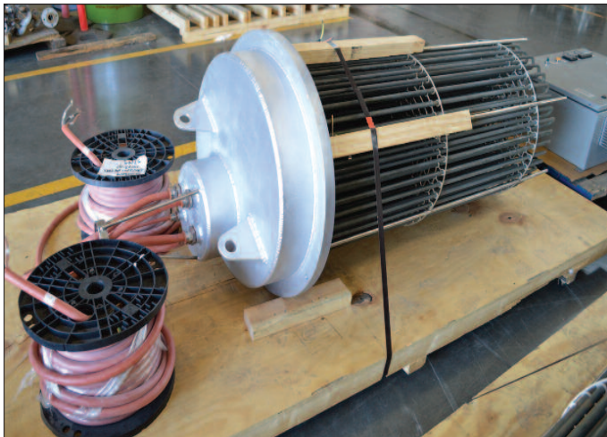
Submersible asphalt heater
