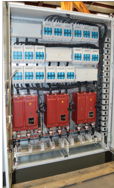
cUL 3200A SCR panel with buss bar
