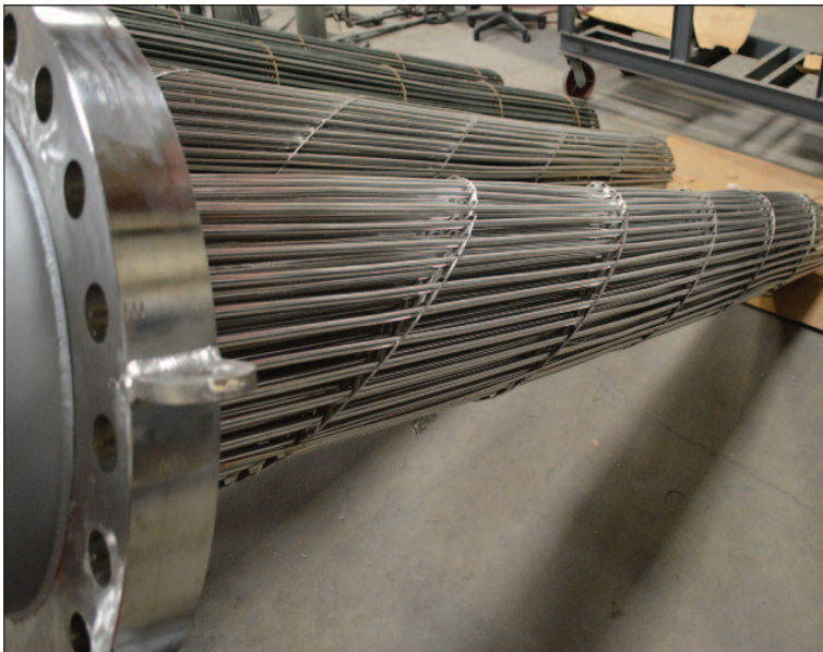
Angled turbulators - optimum heat transfer
